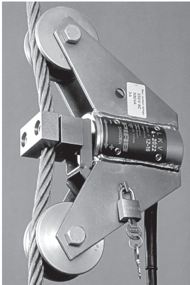
Overload guard LKV with remote display, maximum switching value 1,000 kgf to 16,000 kgf, for line dimension 5-8mm to 40-44mm
